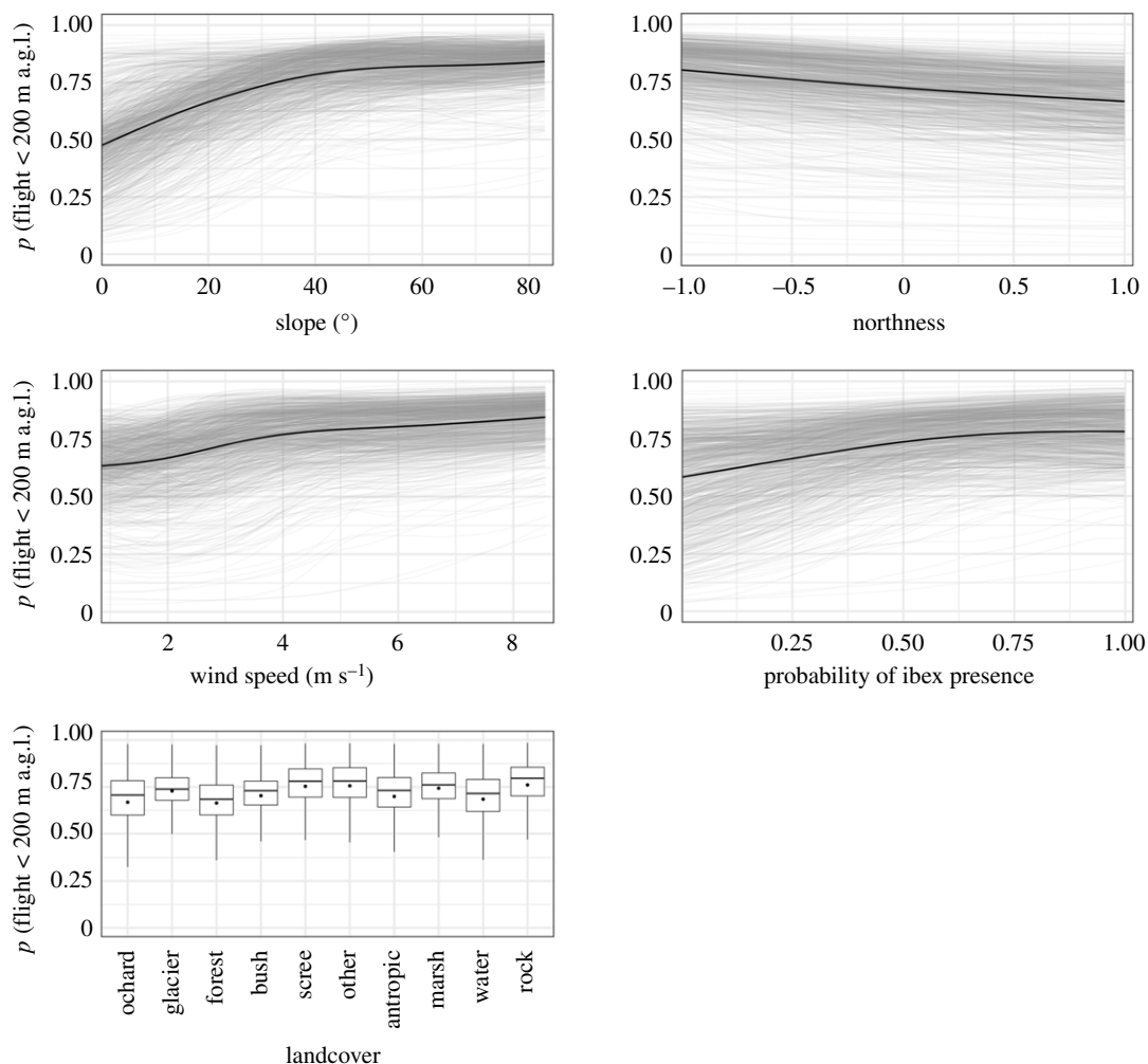
Figure 2. Marginal effect of the five most important environmental variables for predicting the probability of a bearded vulture flying below 200 m.a.g.l. In grey are plotted 1000 randomly sampled individual conditional expectation (ICE) curves [74] and in black the partial dependence (PD) curve [75]. For land cover, a categorical variable, each boxplot shows the ICE values without outliers and the black dot the value of the PD. The curves for the remaining environmental variables are shown in electronic supplementary material, figure S4.
