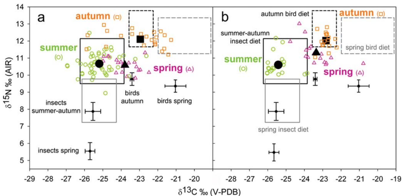
Figure 2. Stable isotope values ( \delta^{13}\text{C} and \delta^{15}\text{N} ) found in bat blood in 2003 (a) and 2004 (b). Individual samples are depicted by small, empty symbols in color, whilst large black symbols show corresponding average group values (seasons are shown with different colours; labelling on both graphs). Mean ( \pm SE) values for potential prey are also shown as small diamonds with bi-directional error bars (labels in 2a). Boxes represent the range of expected values, considering 99% CI for prey and accounting for fractionation factors in the blood of bats that would mirror a pure invertebrate diet (full frames) or a pure bird diet (dashed frames) in spring (grey frames), summer and autumn (black frames, labels in 2b), respectively (see Methods). Partial labelling for prey isotopic signatures («crosses») and expected dietary isotopic signatures (rectangular frames) are shown to enhance clarity.
