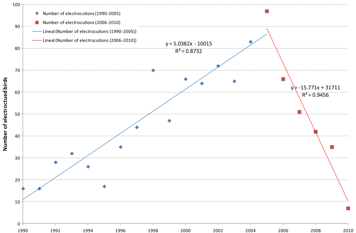
Fig. 2. Regression of the annual mortality index of Spanish ringed species between 1990–2010. Blue line indicates the trend between 1990–2005 and the red line indicates the trend between 2006–2010. (For interpretation of the references to colour in this figure legend, the reader is referred to the web version of this article.)
